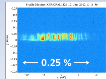
Measured SASE spectrum (LCLS)
